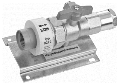
Type 0272 downstream from the house connection
