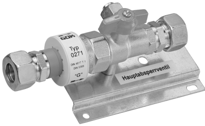
Type 0271 upstream from the house connection
